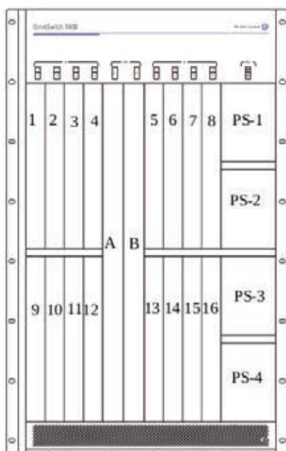
OS9800 (18-Slot Chassis)
