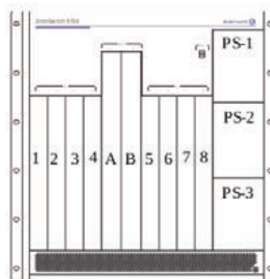
OS9700/OS9702 (10-Slot Chassis)
